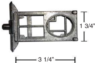
DIE CAST CONCEALED LATCH INSIDE ASSEMBLY
