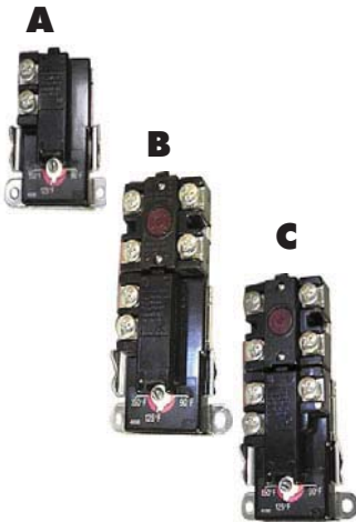
THERMOSTAT CONTROLS FOR WATER HEATER ELEMENTS
